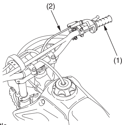
(1) throttle (2) throttle cable
